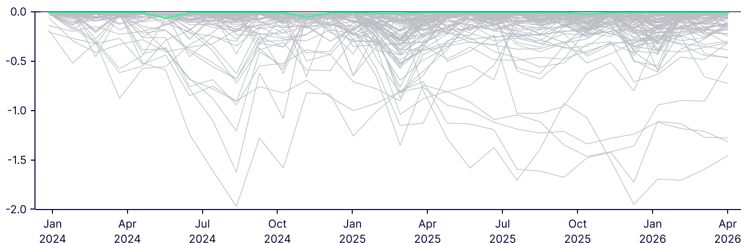
Figure 4: Alpha drawdown by active manager in the US Corporate universe (Jan 2024–June 2026)
